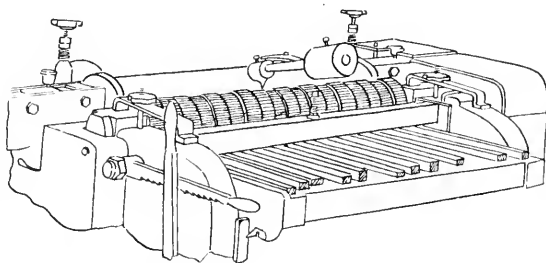
FIG. 153. SECTIONAL FEED ROLLS.
